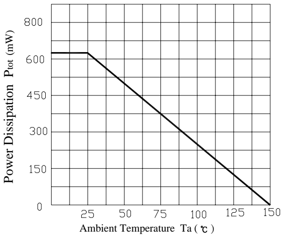
P_{tot} - T_a
